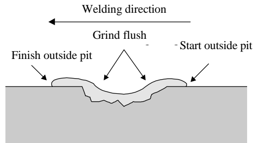
Fig. 6.7. Welding of pits
