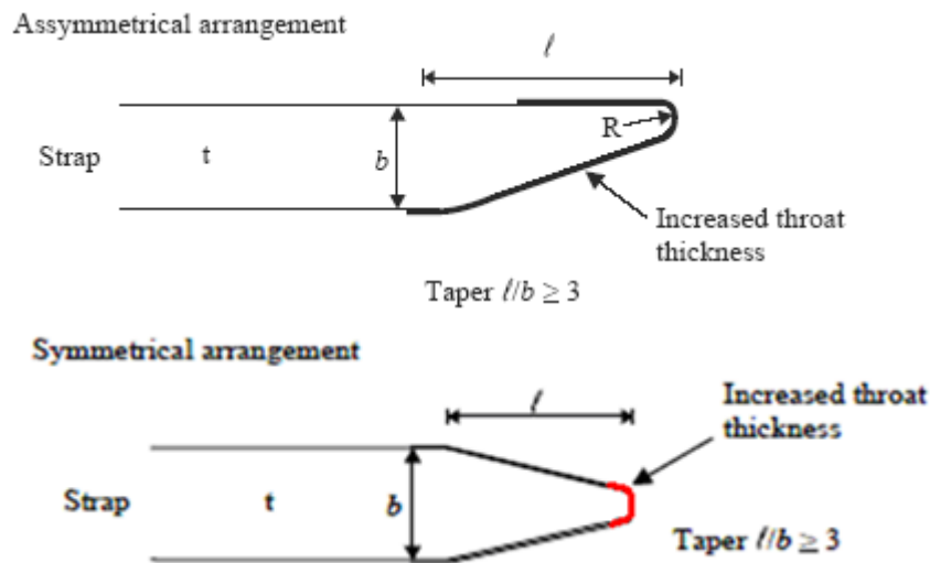
Fig. 6.6 Application of Doubling Straps
