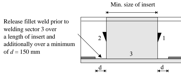
Fig. 6.4. Welding sequence for inserts of stiffeners
