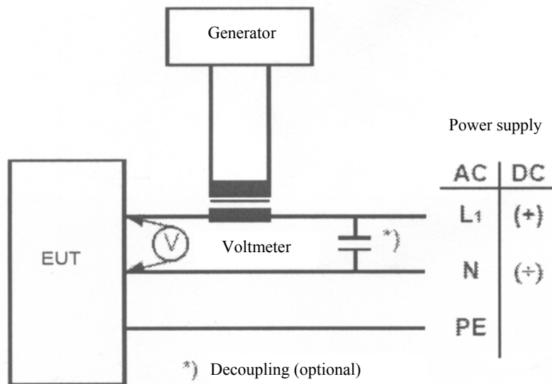
Fig. 2.19. Test set-up – conducted low frequency test
